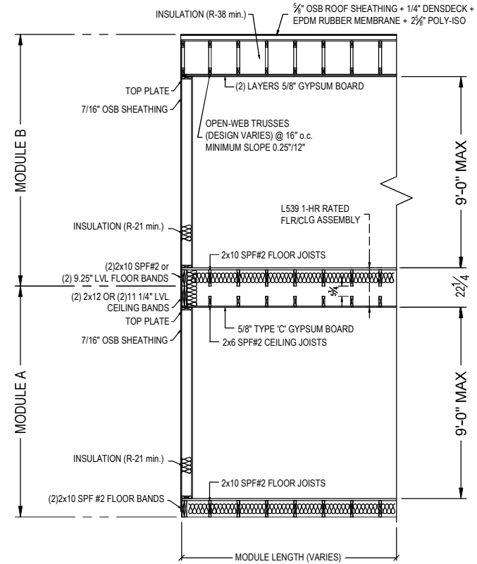
2 4.1 TYPICAL CROSS SECTION VIEW B
