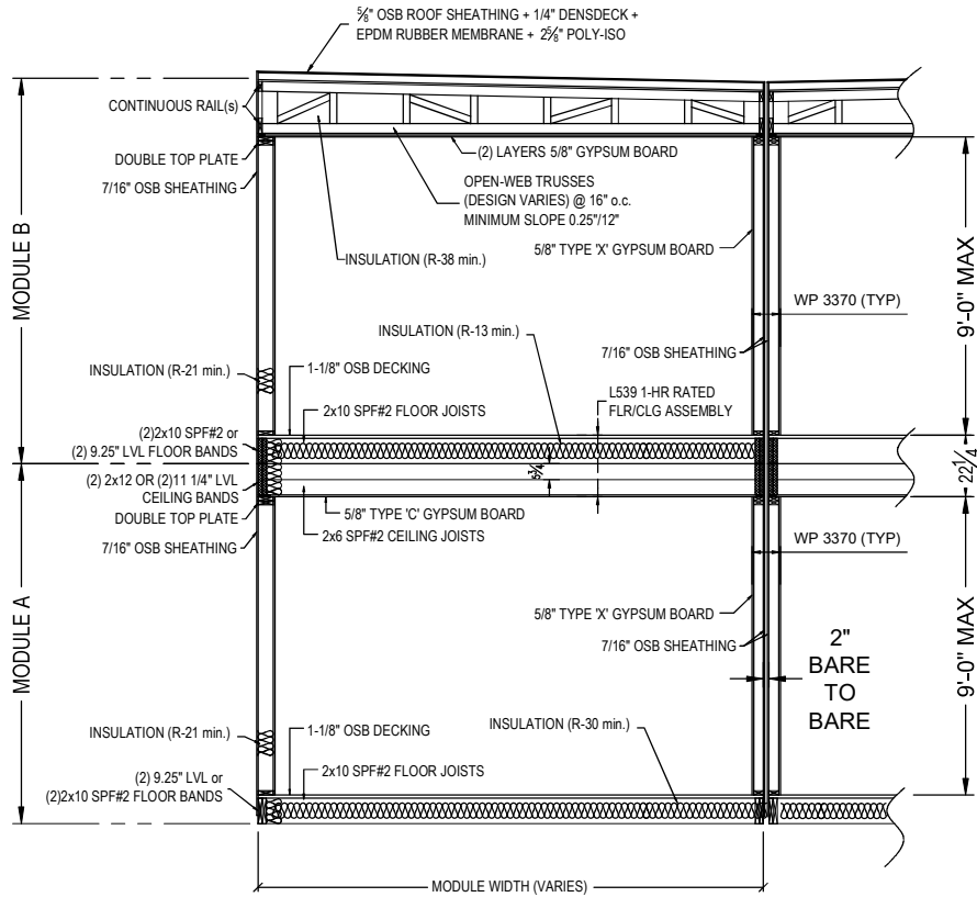
1 4.1 TYPICAL CROSS SECTION VIEW A
