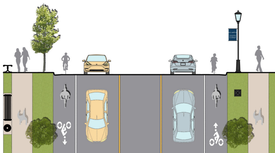
(left) section view, Schematic Alternative 1
